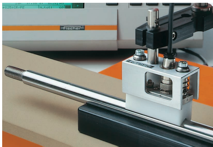
Automated measurement of the chrome coating on piston rods with the probe V2FGA06H.
